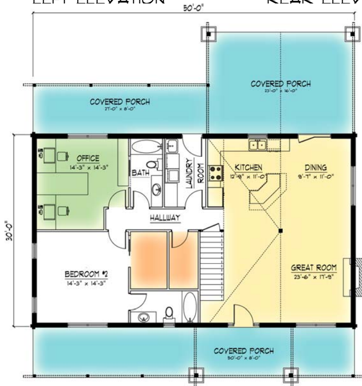
FIRST FLOOR PLAN 1500 SQFT
